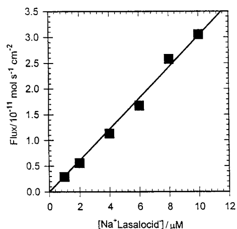
Fig. 4 Flux of ferrioxamine B as a function of membrane phase sodium lasalocid concentration. Source phase: 0.02 M FeHDFB + MeSO 3 - , 0.04 M Mg 2+ , 0.08 M ClO 4 - , pH 9. Membrane phase: 1–10 μM Na + lasalocid - in CHCl 3 . Receiving phase: 0.1 M Na + ClO 4 - , pH 9.
