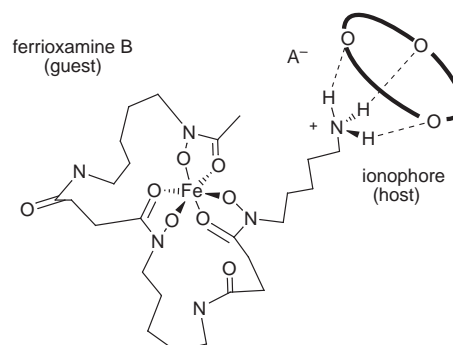
Fig. 1 Siderophore-ionophore assembly formed by second-sphere complexation of ferrioxamine B by an uncharged host.
